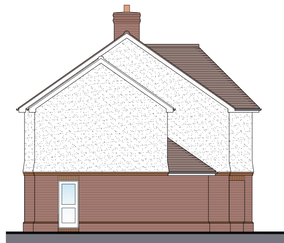
SIDE ELEVATION TYPE C(1:100)
