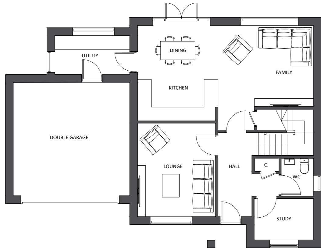
GROUND FLOOR PLAN TYPE D (1:100)
